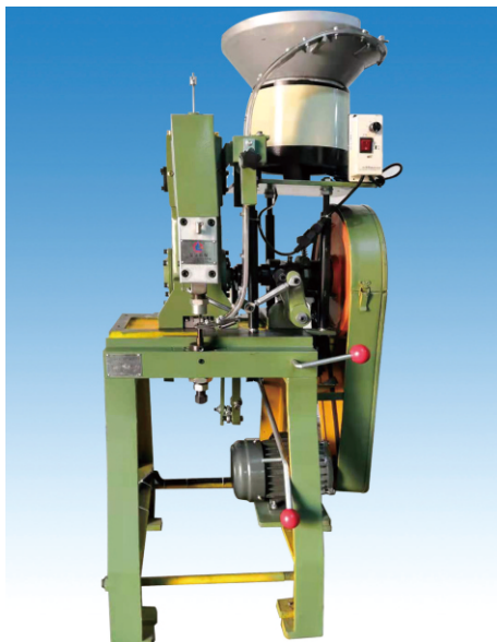
NKJX021 Single-Railway & vibrating Disc Assembled Button Machine Speed: 9600Pcs/H Power: 0.55KW/380V/50HZ Size: 860*880*1500mm Weight: 280Kg
